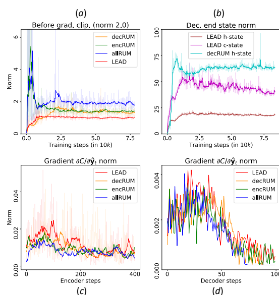
Figure 6: Text summarization study on CNN/Daily Mail . (a) Global norm of the gradients over time; (b) Norm of the last hidden state over time; (c) Encoder gradients of the cost wrt the bi-directional output (400 encoder steps); (d) Decoder gradients of the cost wrt the decoder output (100 decoder steps). Note that (c,d) are evaluated upon convergence, at a specific batch, and the norms for each time step are averaged across the batch and the hidden dimension altogether.
