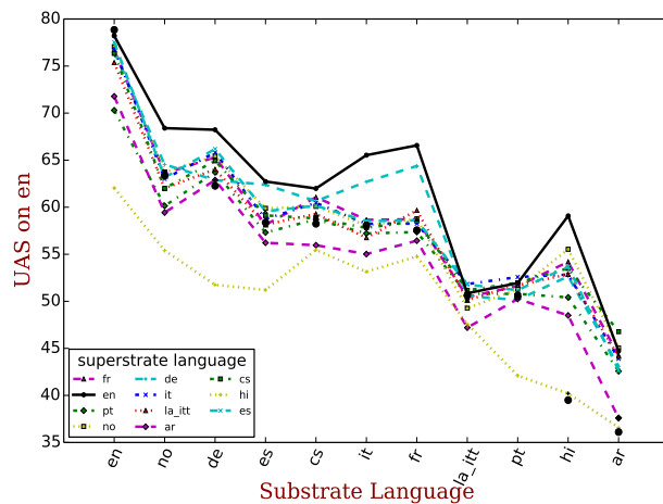
Figure 7: UAS performance of different source parsers when applied to English development sentences. The x axis shows the 10 real training languages S , in decreasing order of their UAS performance (plotted as large black dots). For each superstrate R , we plot a curve showing—for each substrate S —the best UAS of the languages S[R/N] , S[R/V] and S[R/N, R/V] . The points where R = S are specially colored in black; these are instances of self-permutation (§5). We also add “cheating results” where English itself is used as the substrate (left column) and/or the superstrate (solid black line at top). Thus, the large black dot at the upper left is a supervised English parser.
