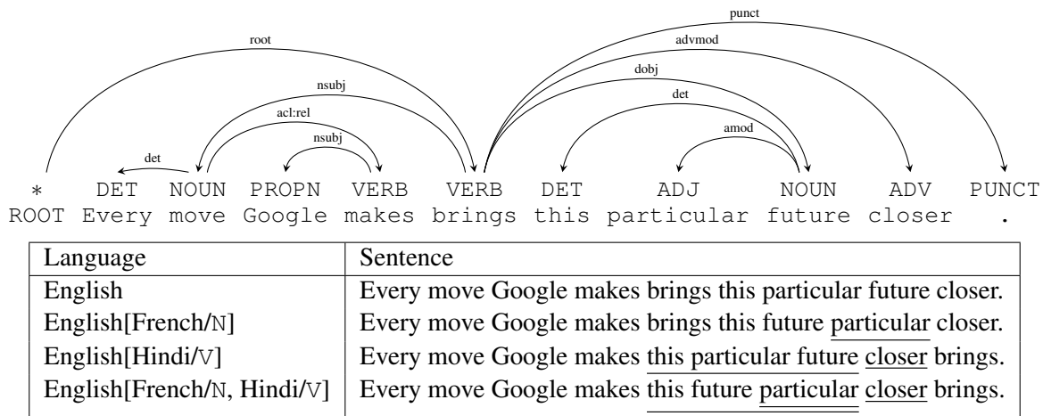
Figure 1: The original UD tree for a short English sentence, and its “translations” into three synthetic languages, which are obtained by manipulating the tree. (Moved constituents are underlined.) Each language has a different distribution over surface part-of-speech sequences.
