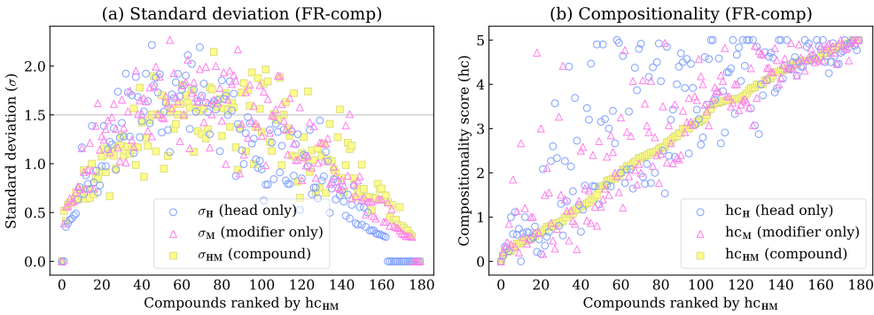
Figure 1 Left: Standard deviations ( \sigma_H , \sigma_M , and \sigma_{HM} ) as a function of hc_{HM} in FR-comp . Right: Average compositionality ( hc_H , hc_M , and hc_{HM} ) as a function of hc_{HM} in FR-comp .
