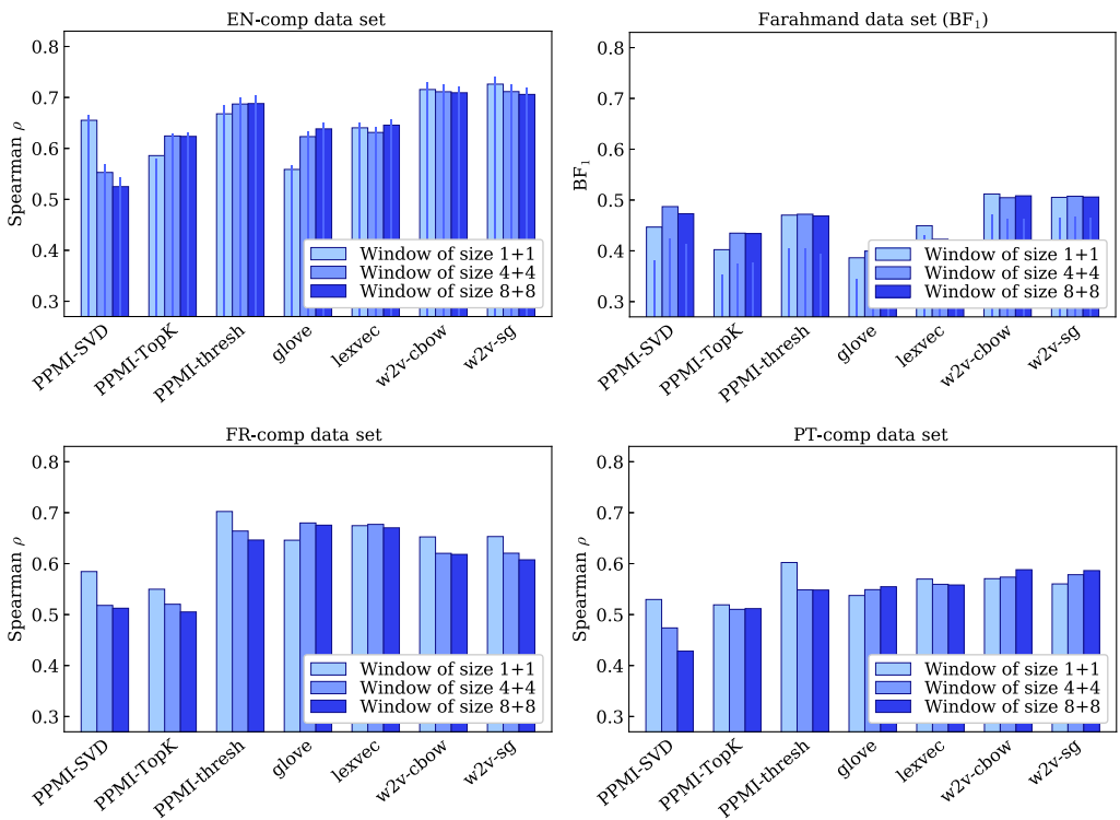
Figure 5 Best results for each DSM and WINDOWSIZE (1+1, 4+4, and 8+8), using BF_1 for Farahmand , and Spearman \rho for other data sets. Thin bars indicate the use of fallback in English. Differences between the two highest Spearman correlations for each model are statistically significant ( p < 0.05 ), except for PPMI-SVD , according to Wilcoxon’s sign-rank test.
