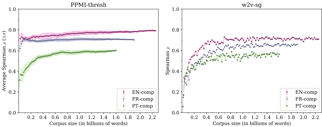
Figure 8 Spearman’s \rho for increasing corpus sizes for PPMI-thresh (left) and w2v-sg (right) for EN-comp in red, FR-comp in blue, and PT-comp in green. Corpus sizes are in the x-axis in billion words. Curves for PPMI-thresh show average and standard deviation (error bars) across 8 samplings of the corpus.
