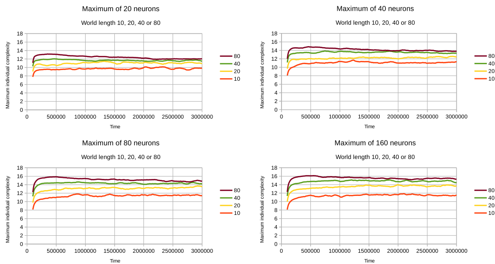
Figure 2. Results when scaling world length (at different maximum numbers of neurons per individual).
