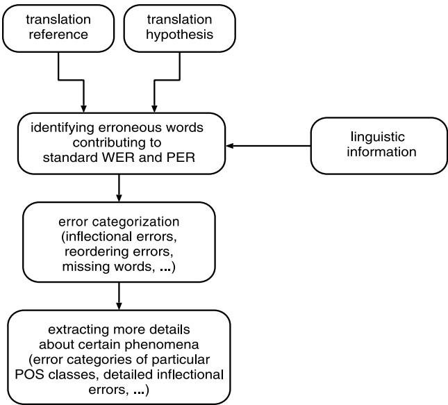
Figure 1 General procedure for automatic error analysis based on the standard word error rates and linguistic information.
