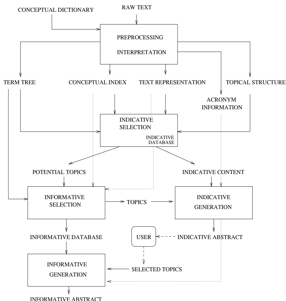
Figure 3 SumUM architecture.
